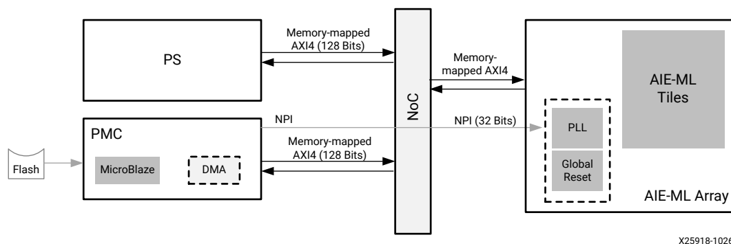
Figure 44: AIE-ML Array Configuration using NoC and NPI
