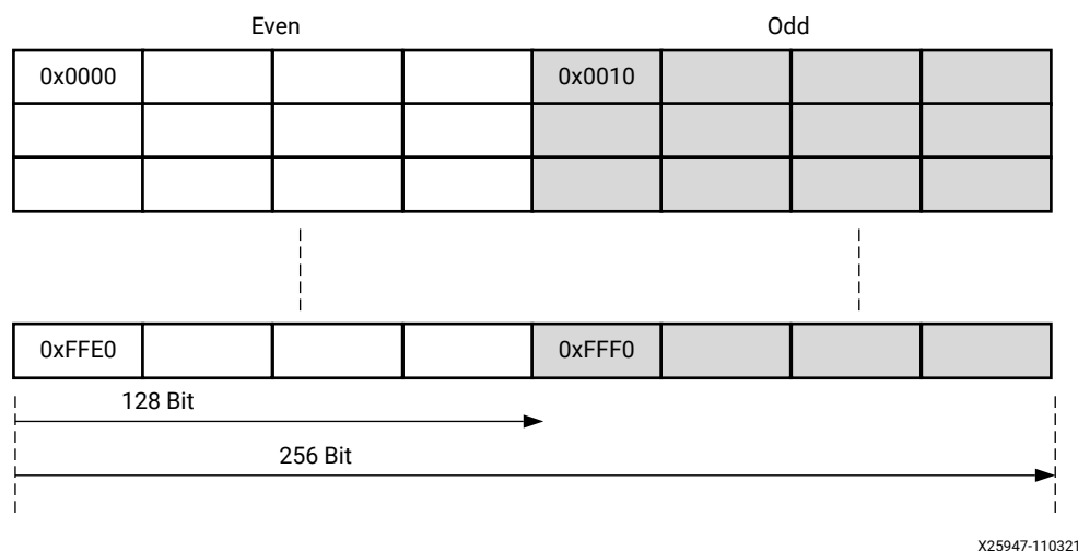
Figure 34: Interleaving in Data Memory (64 KB per Block)
