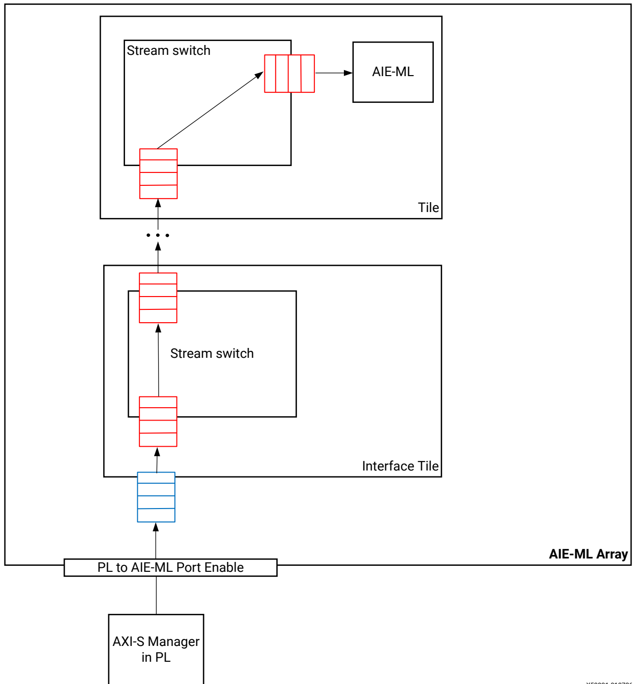
Figure 31: Typical Buffering Stages
