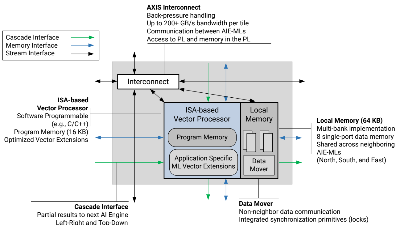
Figure 7: AIE-ML Tile Block Diagram
