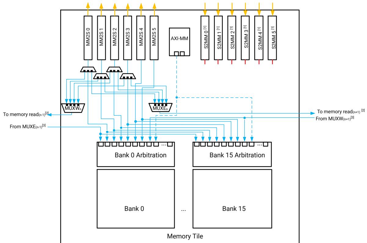
Figure 41: Memory Tile Memory Read Interfaces
