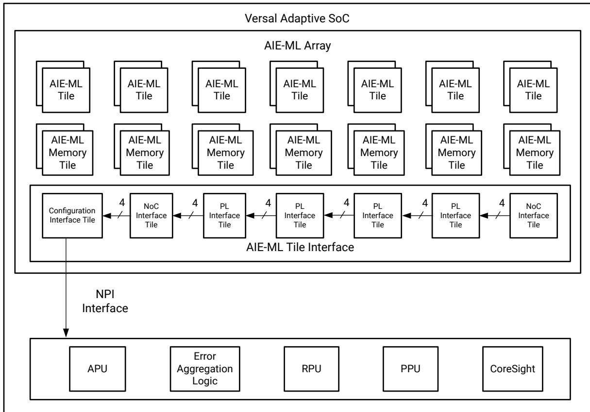
Figure 32: Connecting Interrupts from the AIE-ML Array to Other Functional Blocks
