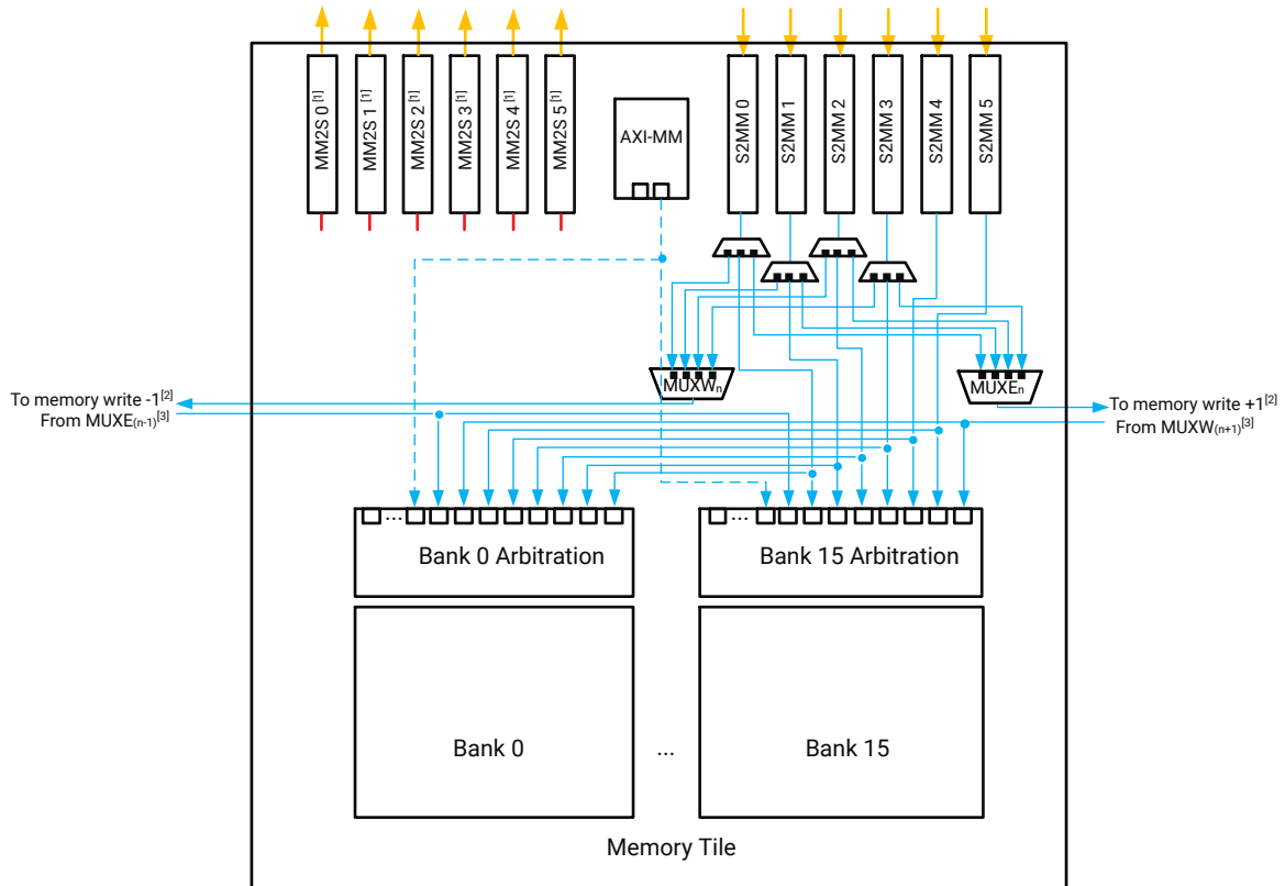
Figure 42: Memory Tile Memory Write Interfaces
